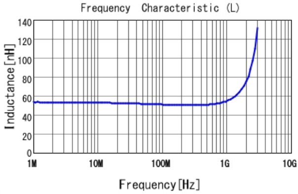
LQW15AN51NJ8Z L
