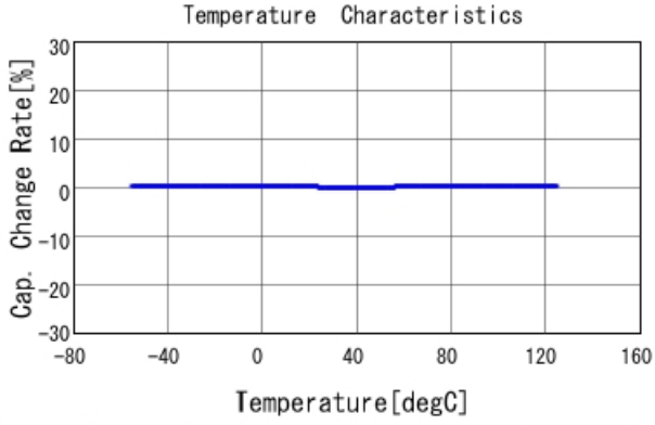
GRM1555C1H5R6DA01 C-Temp. capchange, DCOV, AC1Vrms
