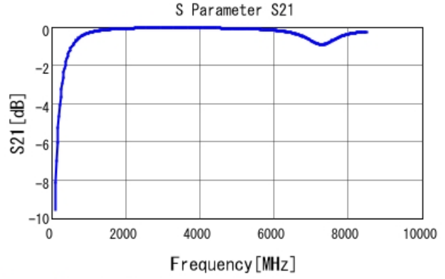
GRM1555C1H5R6DA01 S21 DCOV, 25degC
