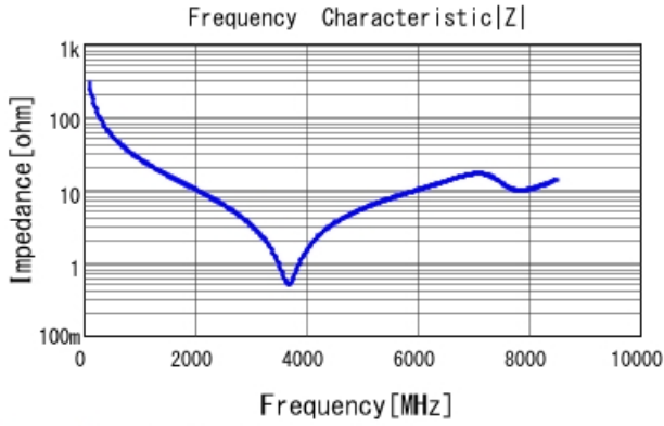
GRM1555C1H5R6DA01 |Z| DCOV, 25degC
