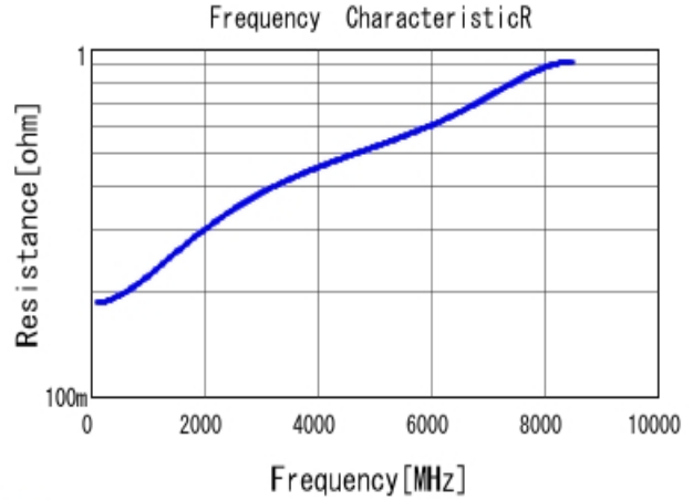
■ GRM0335C1H8R2CA01 R DC0V, 25degC
