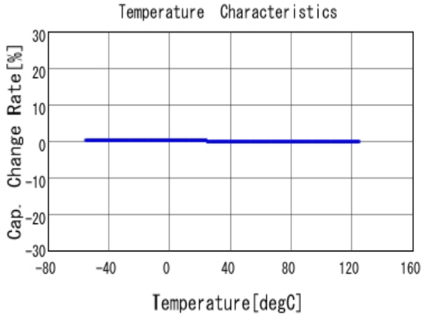
■ GRM0335C1H8R2CA01 C-Temp. capchange, DCOV, AC1Vrms
