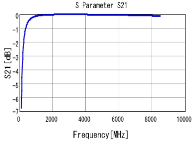
■ GRM0335C1H8R2CA01 S21 DCOV, 25degC
