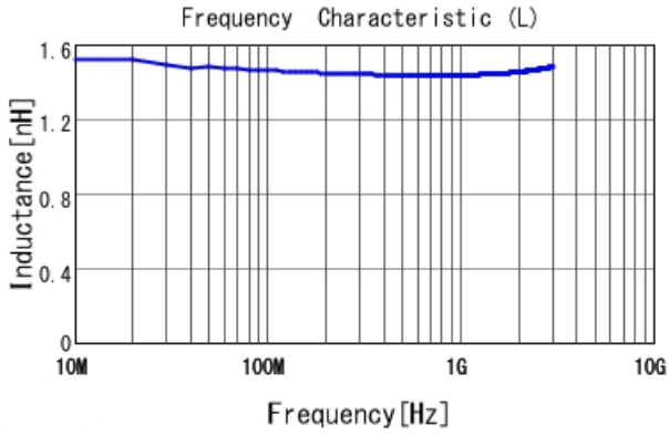
LQP03HQ1N4B02 L
