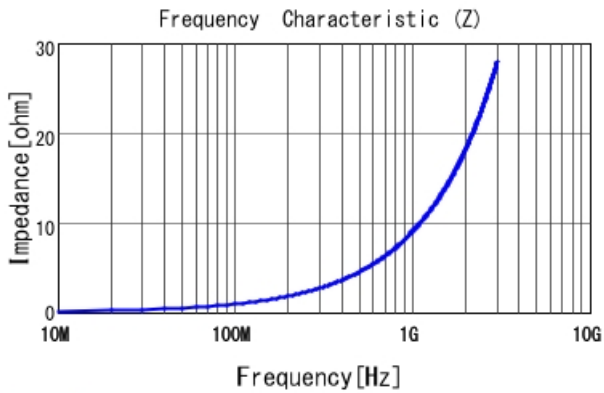
LQP03HQ1N4B02 |Z|
