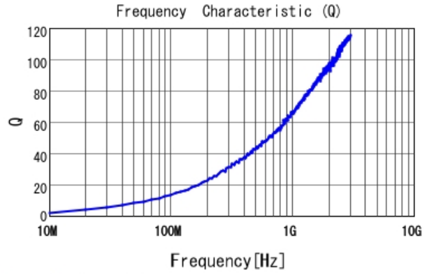
LQP03HQ1N4B02 Q
