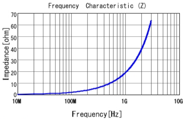
LQP03TG3N0C02 |Z|
