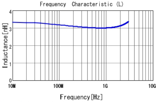
LQP03TG3N0C02 L
