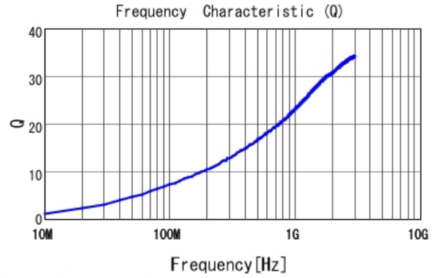
LQP03TG3N0C02 Q
