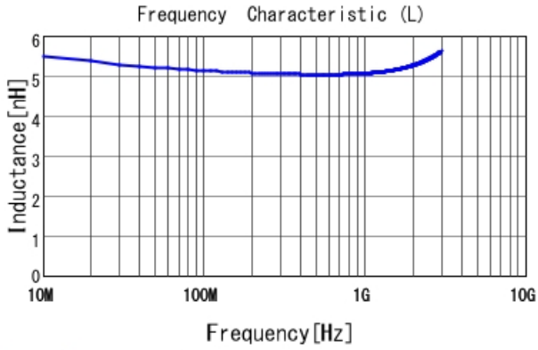
LQW15AN5N2D10 L
