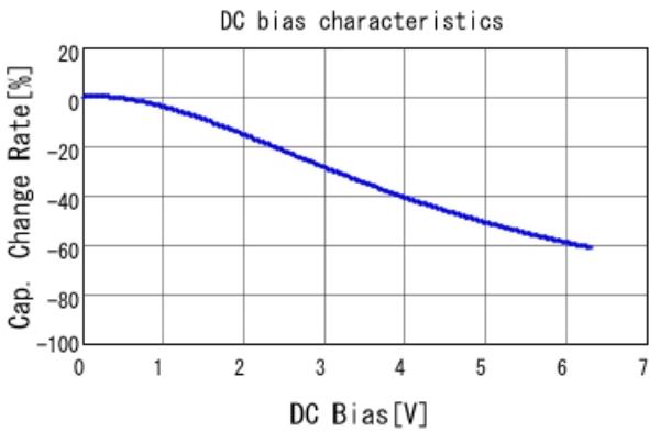
■ GRT31CC80J476KE13 C-DC bias capchange, 25.0degC, AC0.
