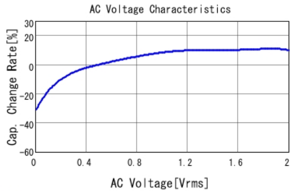
■ GRT31CC80J476KE13 C-AC Voltage capchange, DCOV, 25.0d
