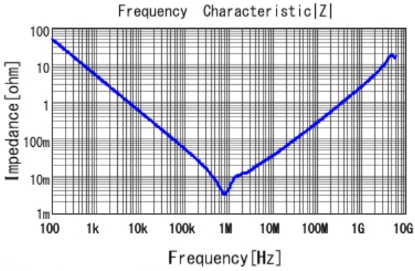
■ GRT31CC80J476KE13 |Z| DCOV, 25degC
