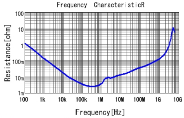
■ GRT31CC80J476KE13 R DCOV, 25degC
