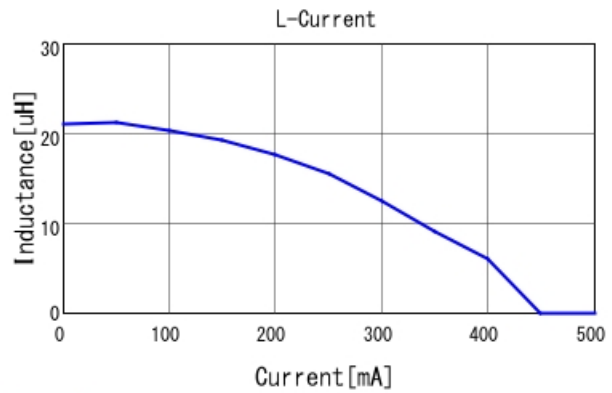
LQH2HPN220MDR L-Current 20degC
