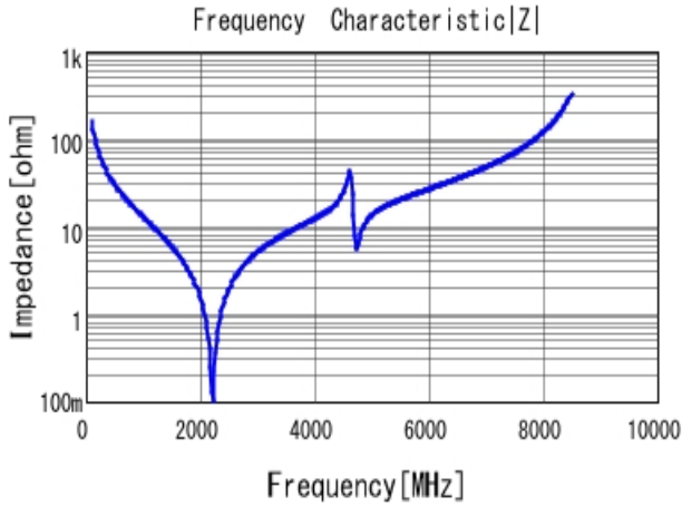
■ GQM2195C2A100GB01 |Z| DCOV, 25degC
