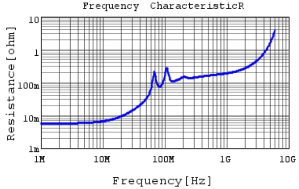
GRM3192C1H333JA01 R DCOV, 20degC
