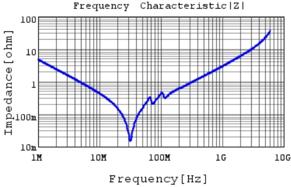
GRM3192C1H333JA01 |Z| DCOV, 20degC
