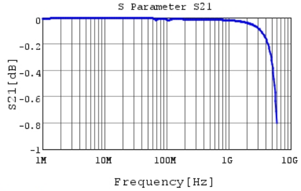
GRM3192C1H333JA01 S21 DCOV, 20degC
