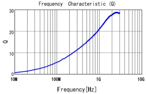
LQP03TG4N7H02 Q
