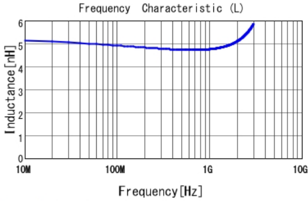
LQP03TG4N7H02 L
