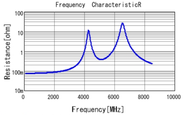
GJM1555C1H220GB01 R DCOV, 25degC
