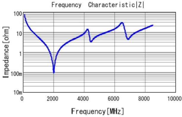
GJM1555C1H220GB01 |Z| DCOV, 25degC
