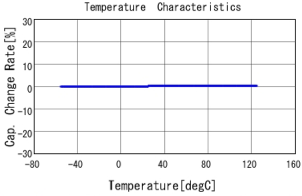
GJM1555C1H220GB01 C-Temp. capchange, DCOV, AC1Vrms
