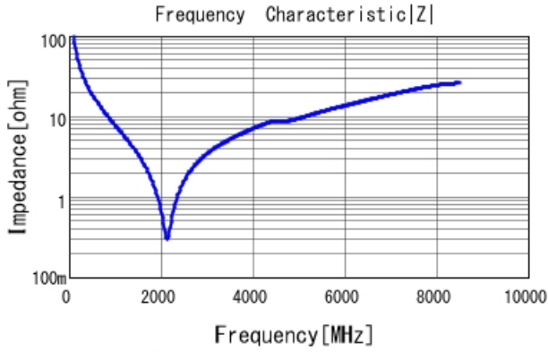
GRM1555C1H160JA01 |Z| DCOV, 25degC
