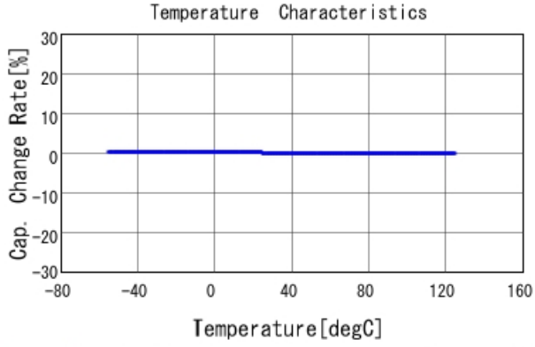
GRM1555C1H160JA01 C-Temp. capchange, DCOV, AC1Vrms
