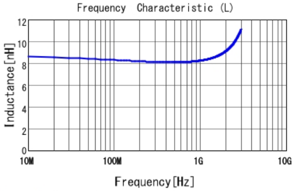
LQP03HQ8N2J02 L
