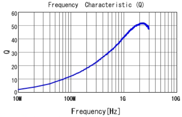
LQP03HQ8N2J02 Q
