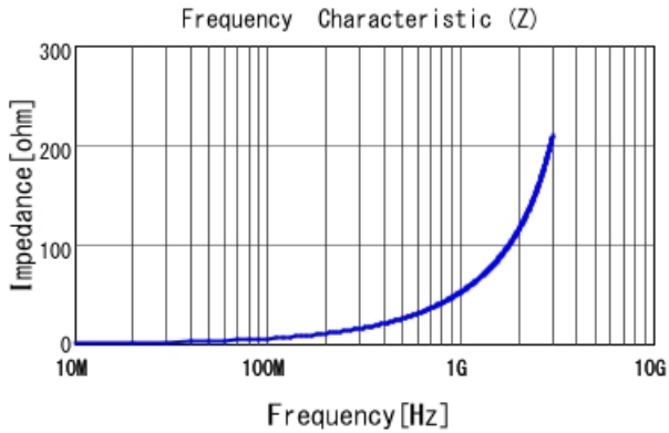
LQP03HQ8N2J02 |Z|
