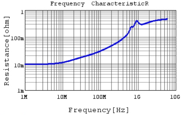
GRM0335C1E102JA01 R DCOV, 25degC
