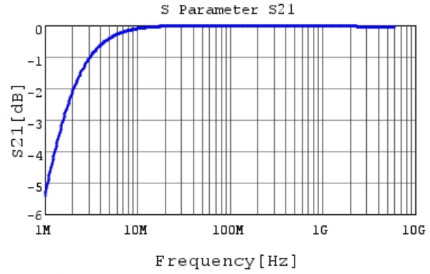
GRM0335C1E102JA01 S21 DCOV, 25degC
