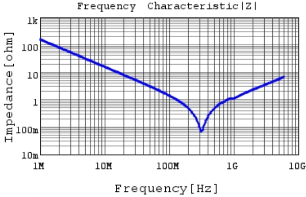
GRM0335C1E102JA01 |Z| DCOV, 25degC
