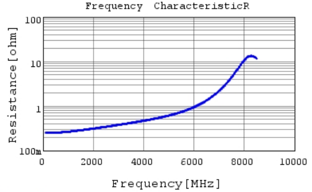
GCM1555C1H4R3CA16 R DC0V, 25degC
