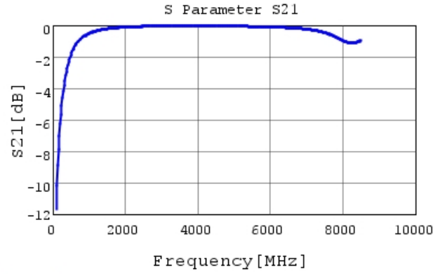
GCM1555C1H4R3CA16 S21 DCOV, 25degC
