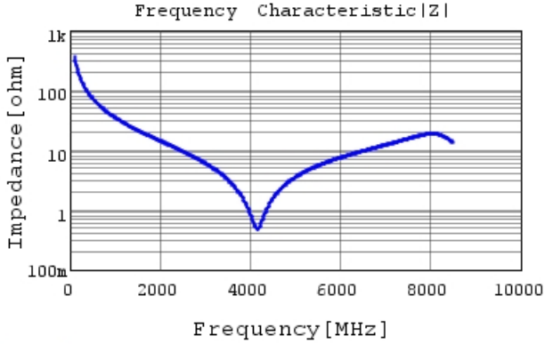
GCM1555C1H4R3CA16 |Z| DC0V, 25degC
