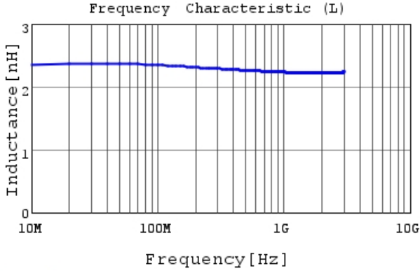
LQP02HQ2N3B02 L
