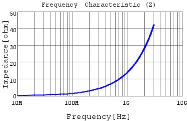
LQP02HQ2N3B02 |Z|
