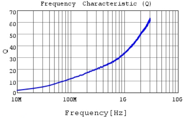
LQP02HQ2N3B02 Q
