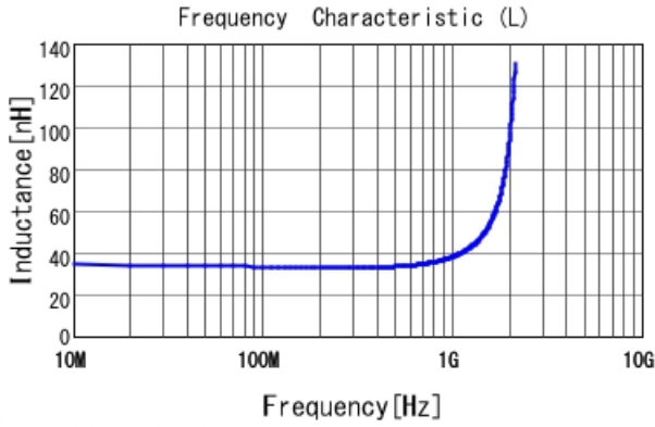
LQP03TN33NJ02 L
