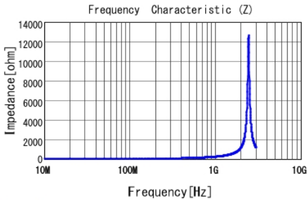
LQP03TN33NJ02 |Z|
