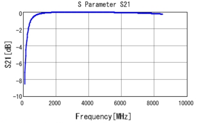
GJM1555C1H6R4BB01 S21 DC0V, 25degC
