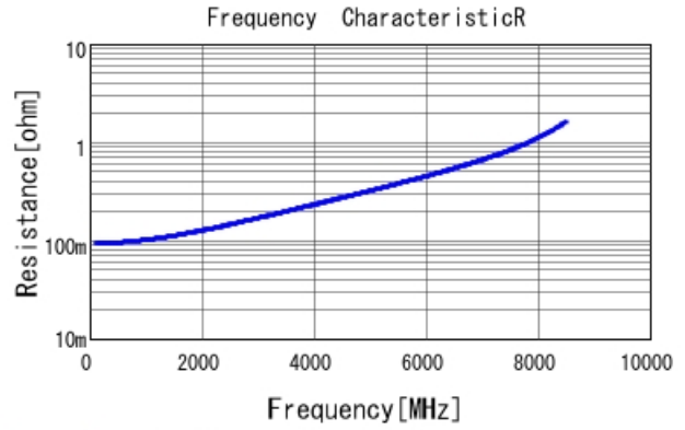
GJM1555C1H6R4BB01 R DCOV, 25degC
