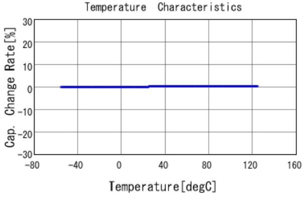
GJM1555C1H6R4BB01 C-Temp. capchange, DC0V, AC1Vrms
