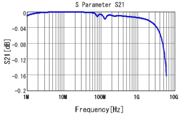
GRM2165C1H333GA01 S21 DCOV, 25degC
