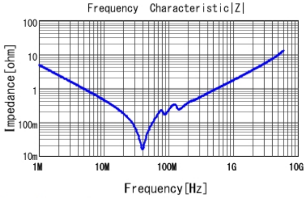
GRM2165C1H333GA01 |Z| DCOV, 25degC
