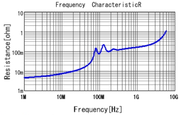
GRM2165C1H333GA01 R DCOV, 25degC
