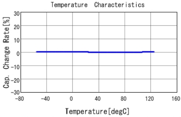
GRM2165C1H333GA01 C-Temp. capchange, DCOV, AC1Vrms
