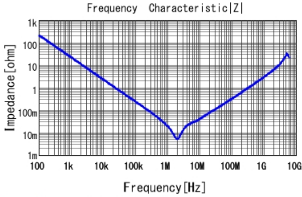
GRM319B30J106KE18 |Z| DCOV, 20degC
