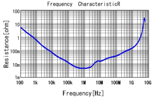
GRM319B30J106KE18 R DCOV, 20degC
