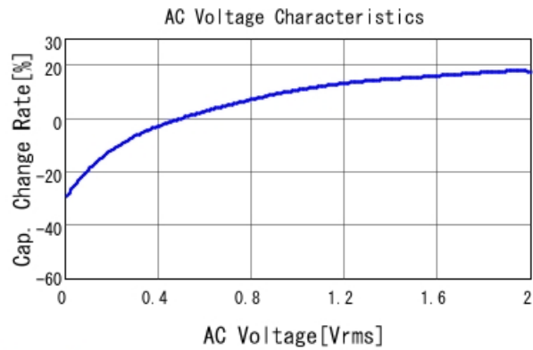
GRM319B30J106KE18 C-AC Voltage capchange, DCOV, 2C
