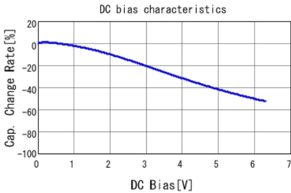
GRM319B30J106KE18 C-DC bias capchange, 20.0degC, A
