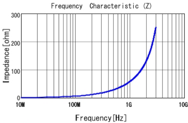
LQP03TN9N1H02 |Z|
