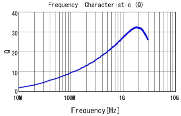
LQP03TN9N1H02 Q
