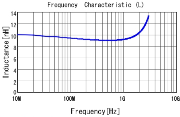
LQP03TN9N1H02 L
