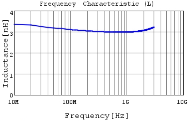
LQP03TQ3N0C02 L
