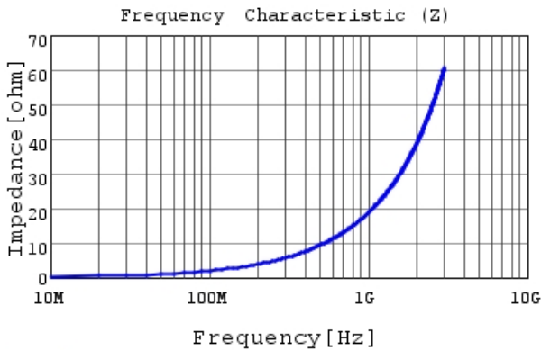
LQP03TQ3N0C02 |Z|
