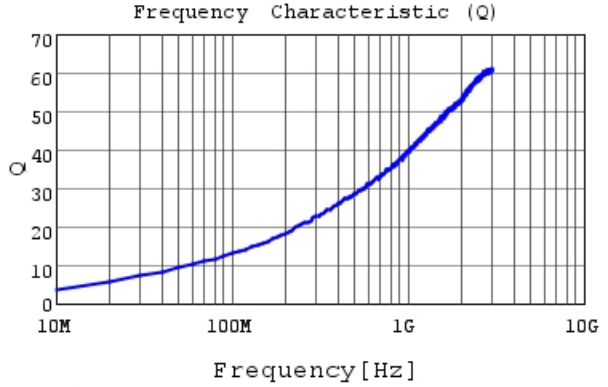
LQP03TQ3N0C02 Q
