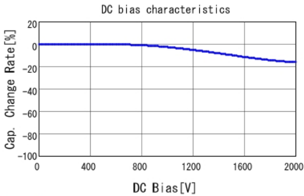
GR442QR73D101KW01 C-DC bias capchange, 25.0degC, A
