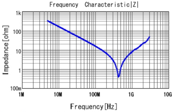
GR442QR73D101KW01 |Z| DCOV, 25degC
