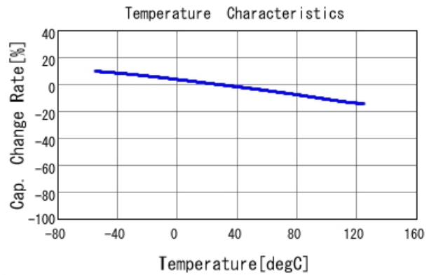
GR442QR73D101KW01 C-Temp. capchange, DCOV, AC1Vrms
