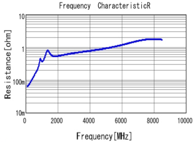
■ GRM1555C1H391JA01 R DC0V, 25degC
