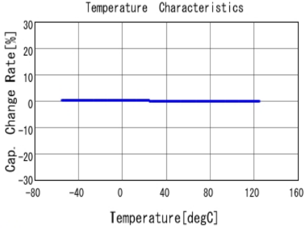
■ GRM1555C1H391JA01 C-Temp. capchange, DCOV, AC1Vrms
