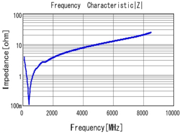
■ GRM1555C1H391JA01 |Z| DC0V, 25degC
