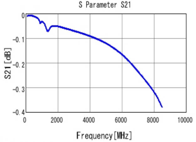
■ GRM1555C1H391JA01 S21 DCOV, 25degC
