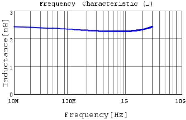
LQG15WH2N3C02 L
