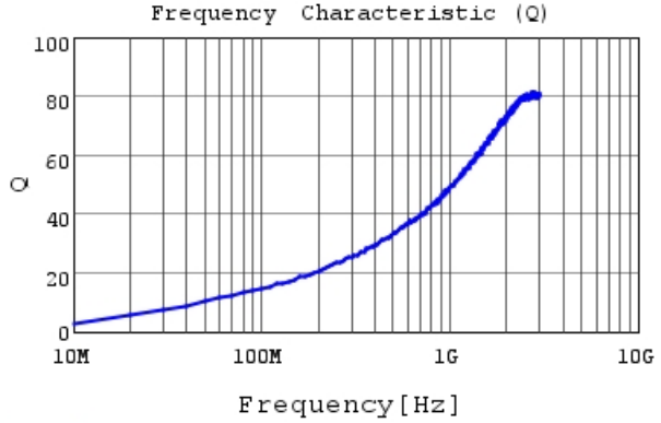
LQG15WH2N3C02 Q
