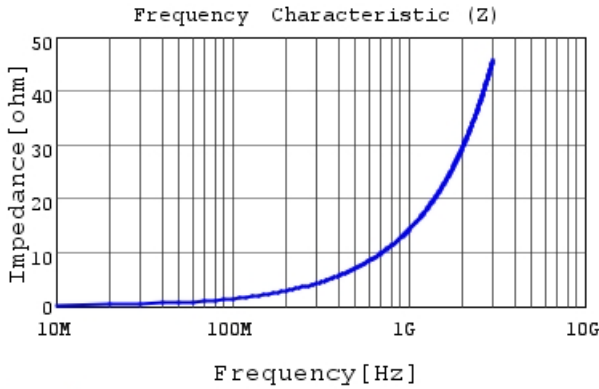
LQG15WH2N3C02 |Z|
