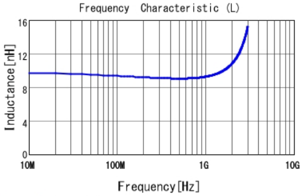
LQP03TG9N1J02 L
