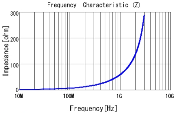
LQP03TG9N1J02 |Z|
