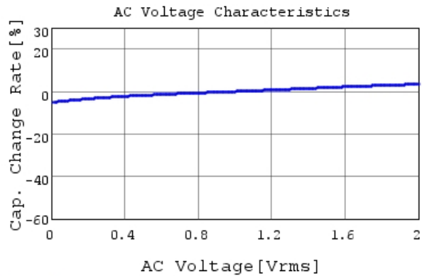
GRM033R71E222MA12 C-AC Voltage capchange, Dc
