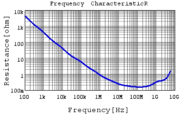
GRM033R71E222MA12 R DCOV, 25degC
