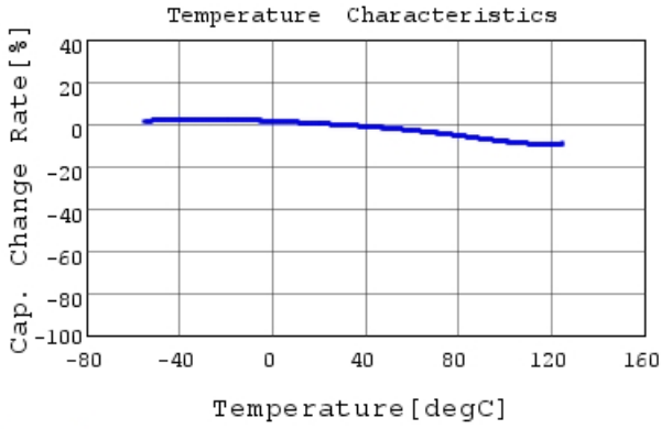
GRM033R71E222MA12 C-Temp. capchange, DC0.0V,
