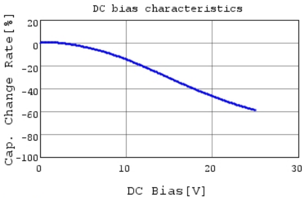
GRM033R71E222MA12 C-DC bias capchange, 25.0c
