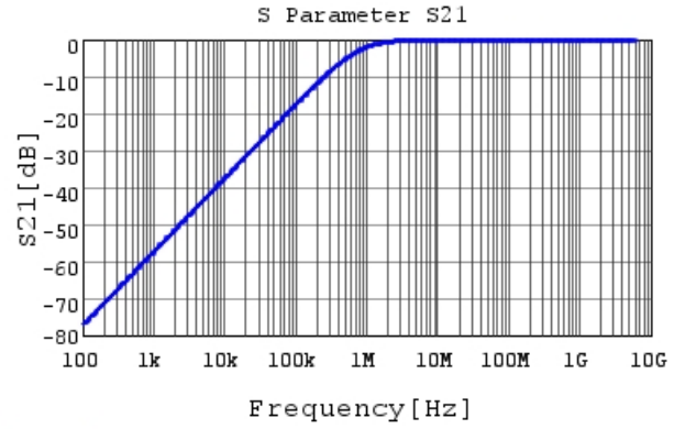
GRM033R71E222MA12 S21 DC0V,25degC
