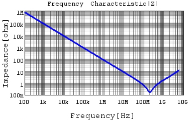
GRM033R71E222MA12 |Z| DCOV, 25degC
