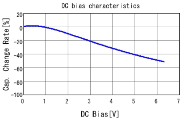
GRM32EB30J476ME16 C-DC bias capchange, 20.0degC, A
