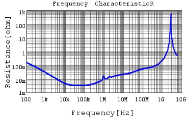
KCM55WR71E476MH01 R DCOV, 25degC
