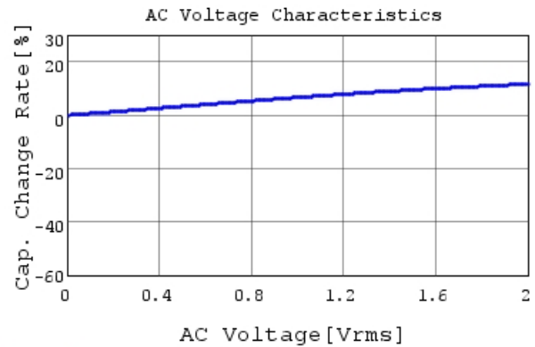
KCM55WR71E476MH01 C-AC Voltage capchange, Dc
