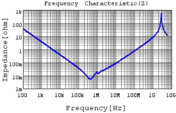
KCM55WR71E476MH01 |Z| DCOV, 25degC
