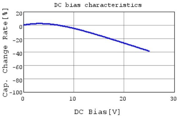
KCM55WR71E476MH01 C-DC bias capchange, 25.0c
