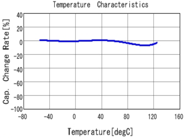
■ GRM155R71H331KA01 C-Temp. capchange, DCO. 0V, AC1.0V rm
