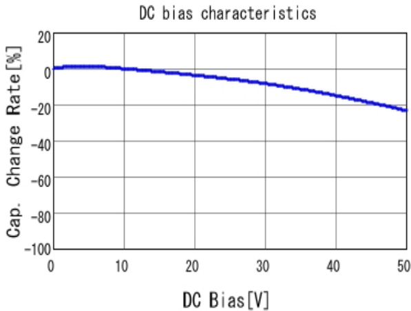
■ GRM155R71H331KA01 C-DC bias capchange, 25.0degC, AC1.
