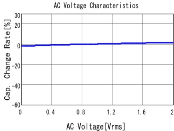
■ GRM155R71H331KA01 C-AC Voltage capchange, DCOV, 25.0d
