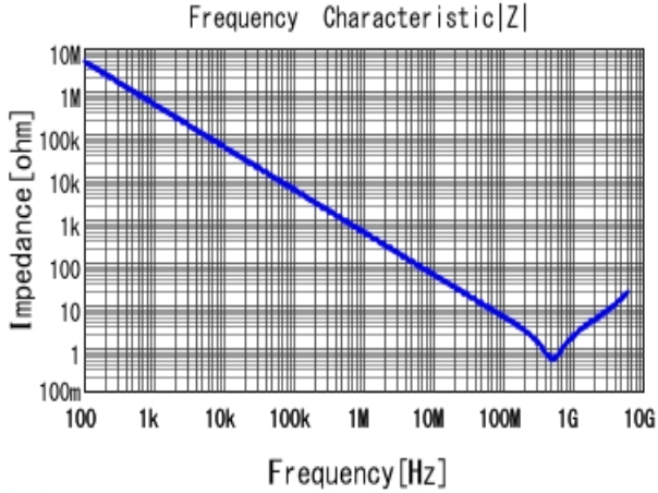
■ GRM155R71H331KA01 |Z| DCOV, 25degC
