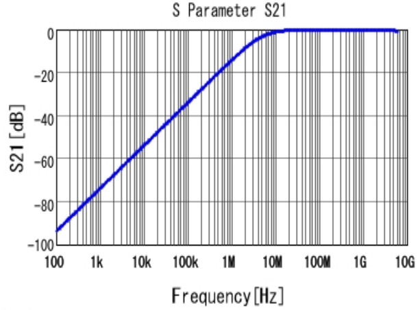
■ GRM155R71H331KA01 S21 DCOV, 25degC
