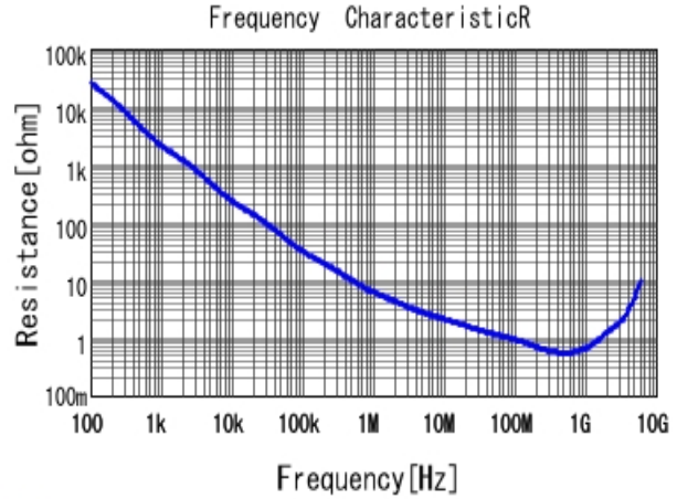
■ GRM155R71H331KA01 R DCOV, 25degC
