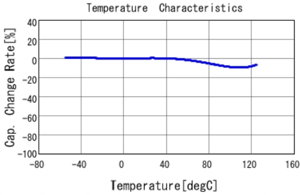
GRM188R71H222JA01 C-Temp. capchange, DC0.0V, AC1.C
