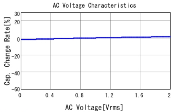
GRM188R71H222JA01 C-AC Voltage capchange, DCOV, 25
