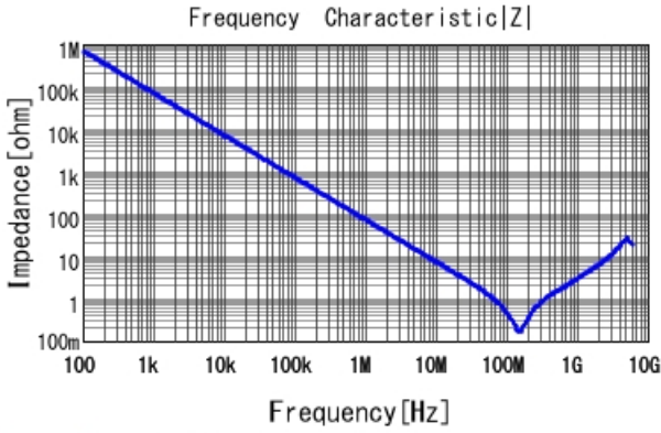
GRM188R71H222JA01 |Z| DCOV, 25degC
