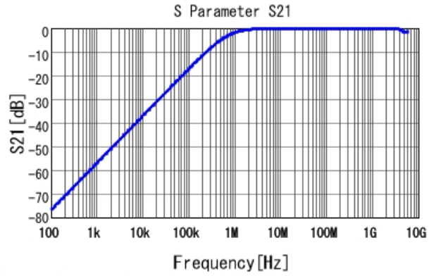
GRM188R71H222JA01 S21 DC0V, 25degC
