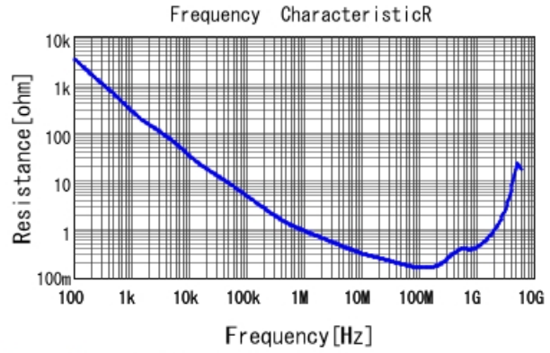
GRM188R71H222JA01 R DCOV, 25degC
