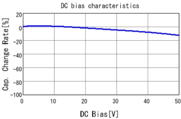
GRM188R71H222JA01 C-DC bias capchange, 25.0degC, A
