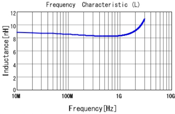
LQP03TN8N2JZ2 L
