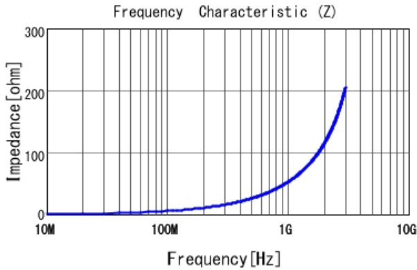
LQP03TN8N2JZ2 |Z|
