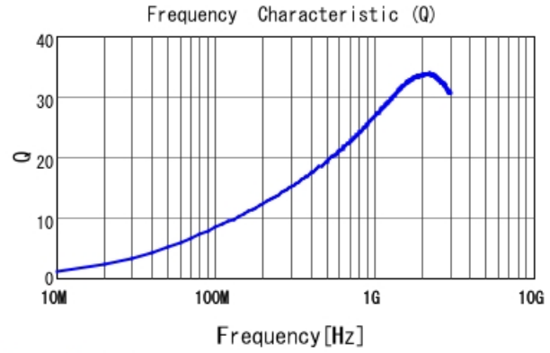
LQP03TN8N2JZ2 Q
