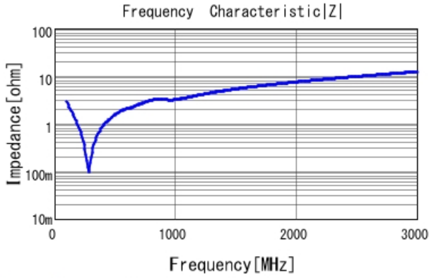
GRM21A7U2E471JW31 |Z| DCOV, 25degC
