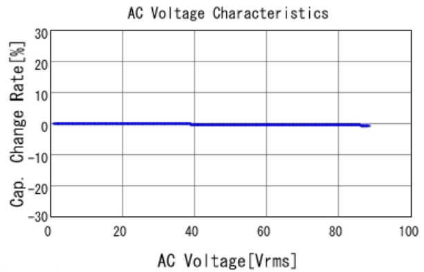
GRM21A7U2E471JW31 C-AC Voltage capchange, DCOV, 25
