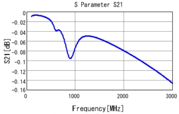
GRM21A7U2E471JW31 S21 DC0V, 25degC
