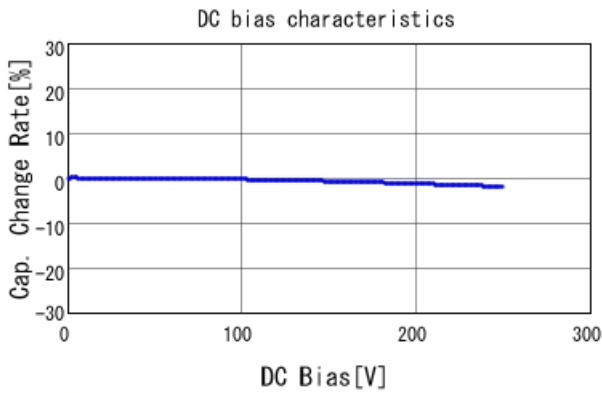
GRM21A7U2E471JW31 C-DC bias capchange, 25.0degC, A
