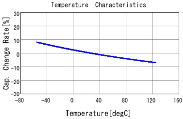
GRM21A7U2E471JW31 C-Temp. capchange, DC0V, AC1Vrms
