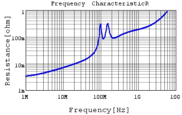
GRM21B5C1H183JA01 R DCOV, 25degC
