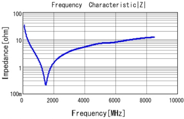
GCM0335C1E470JA16 |Z| DC0V, 25degC
