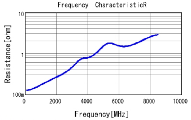
GCM0335C1E470JA16 R DC0V, 25degC
