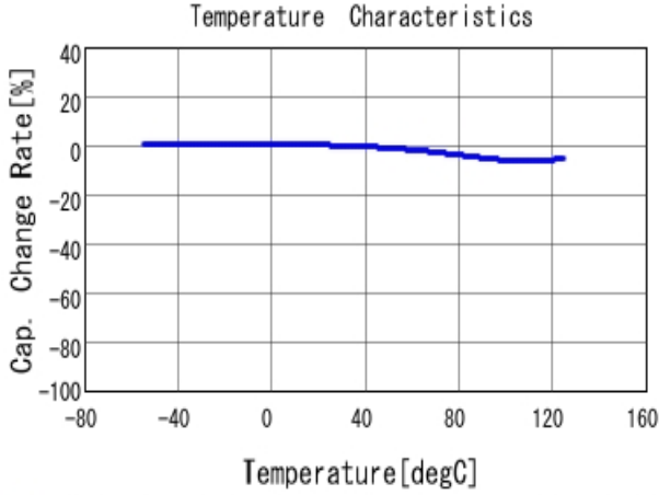
■ GRM033R71H681MA12 C-Temp. capchange, DCO. 0V, AC1.0Vrm
