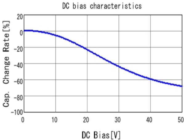
■ GRM033R71H681MA12 C-DC bias capchange, 25.0degC, AC1.
