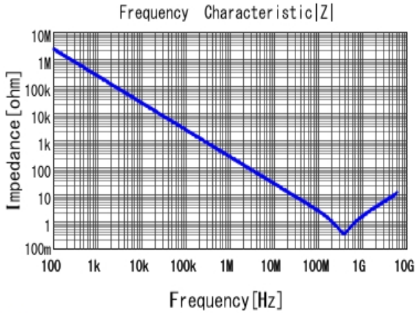
■ GRM033R71H681MA12 |Z| DCOV, 25degC
