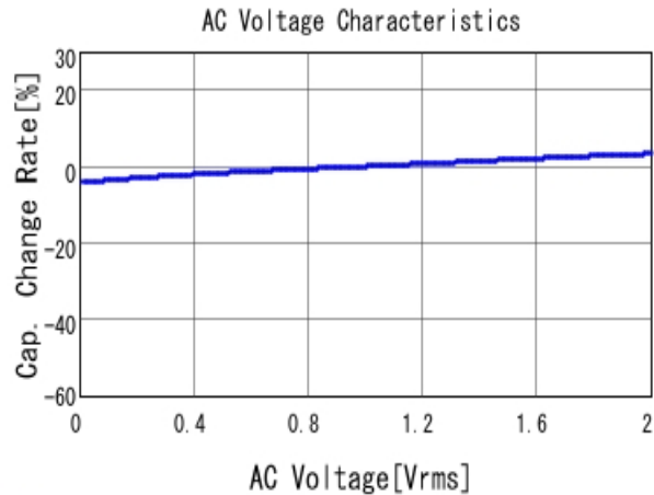
■ GRM033R71H681MA12 C-AC Voltage capchange, DCOV, 25.0d
