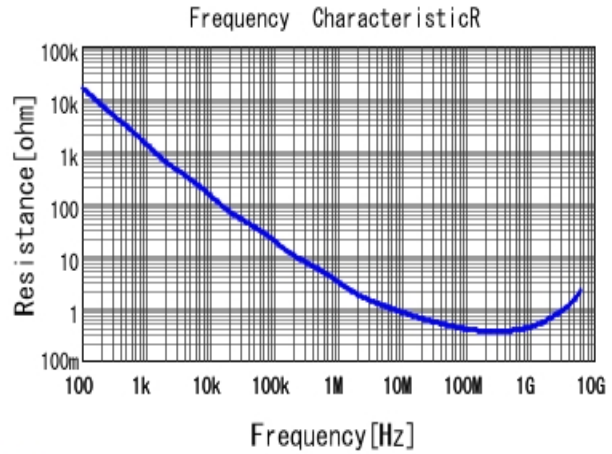
■ GRM033R71H681MA12 R DCOV, 25degC
