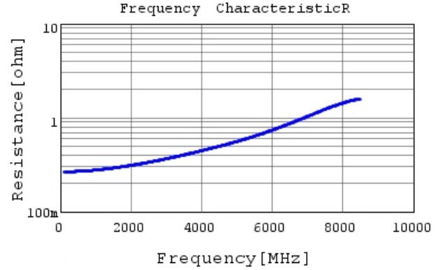
GRM0335C1H2R4BA01 R DCOV, 25degC
