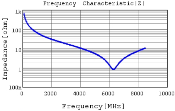
GRM0335C1H2R4BA01 |Z| DCOV, 25degC
