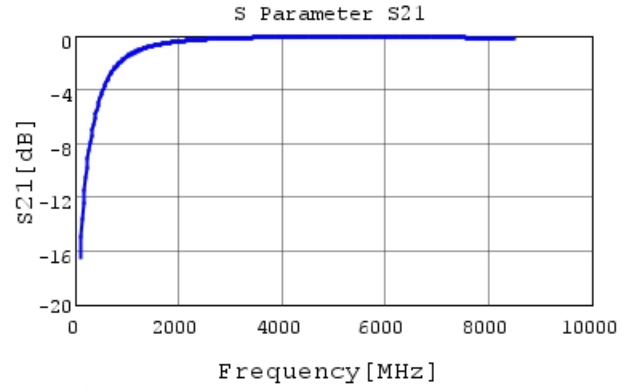
GRM0335C1H2R4BA01 S21 DCOV, 25degC
