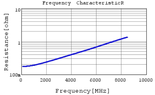
GRM0225C1E330JA02 R DCOV, 25degC
