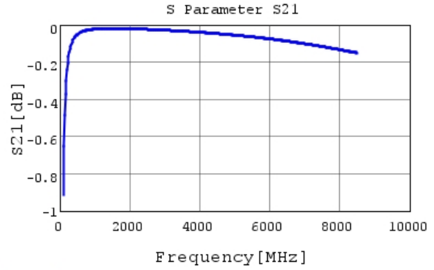
GRM0225C1E330JA02 S21 DCOV, 25degC
