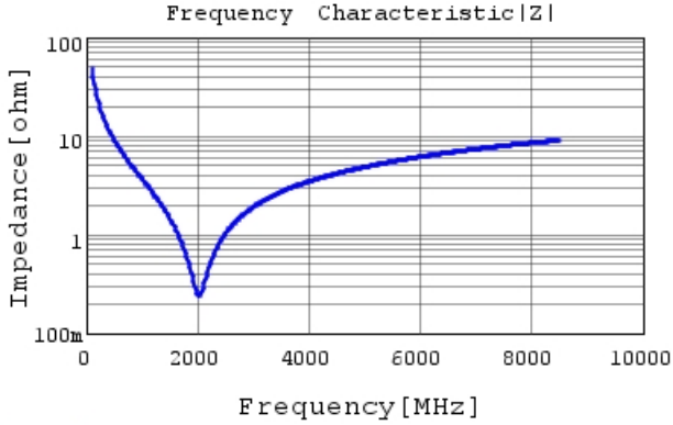
GRM0225C1E330JA02 |Z| DCOV, 25degC
