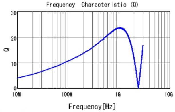
LQG15HS22NG02 Q
