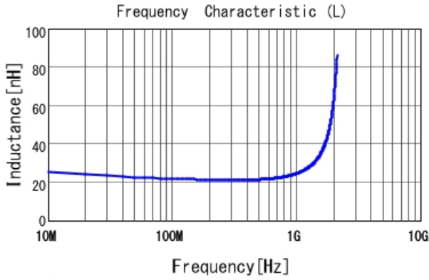
LQG15HS22NG02 L
