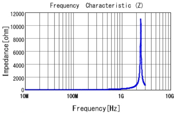
LQG15HS22NG02 |Z|
