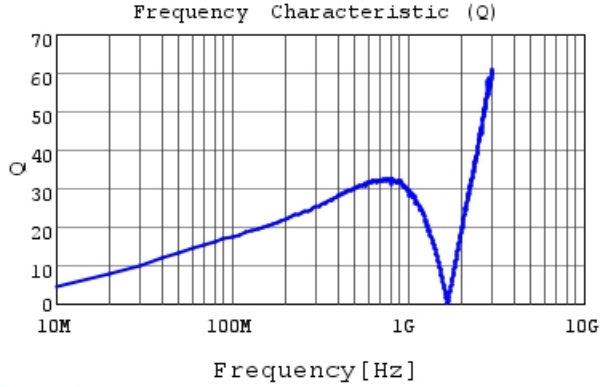
LQG15WH62NG02 Q
