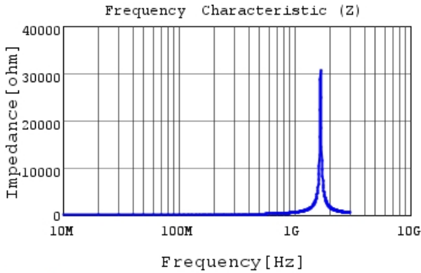
LQG15WH62NG02 |Z|
