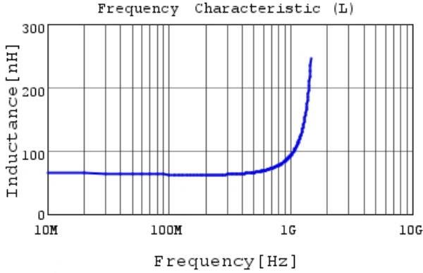
LQG15WH62NG02 L
