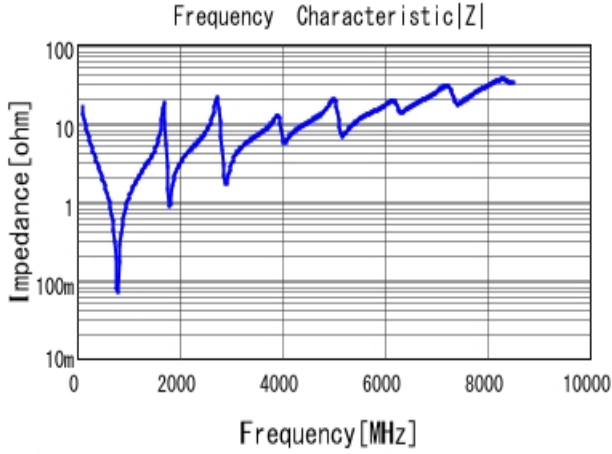
■ GQM2195C2E101GB12 |Z| DCOV, 25degC
