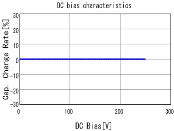
■ GQM2195C2E101GB12 C-DC bias capchange, 25.0degC, AC1V
