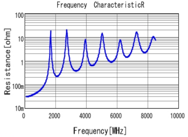
■ GQM2195C2E101GB12 R DCOV, 25degC
