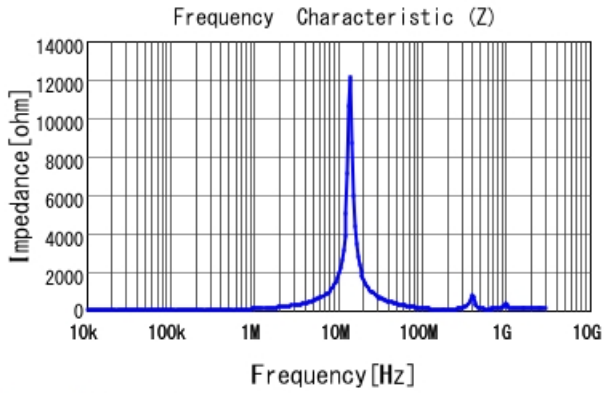
#B953AS-150M=P3 |Z|
