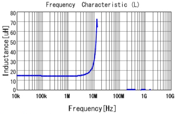
#B953AS-150M=P3 L
