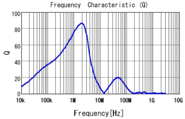
#B953AS-150M=P3 Q
