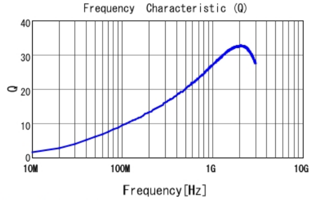
LQP03TN10NJZ2 Q
