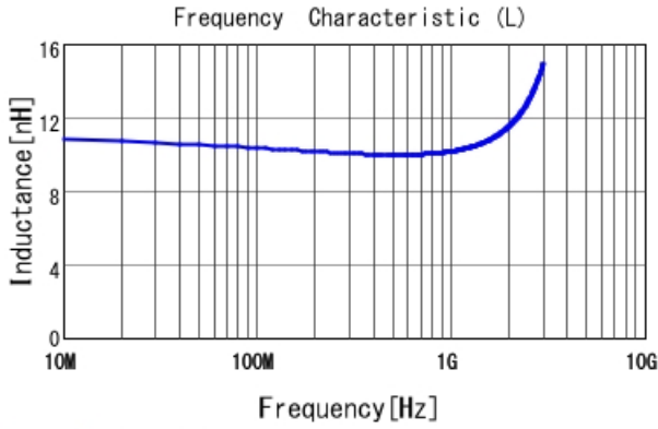
LQP03TN10NJZ2 L
