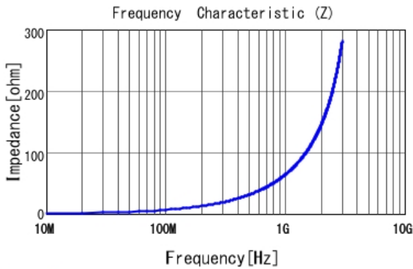
LQP03TN10NJZ2 |Z|
