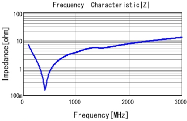
GRM21A7U2E221JW31 |Z| DCOV, 25degC
