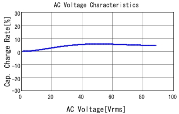
GRM21A7U2E221JW31 C-AC Voltage capchange, DCOV, 25
