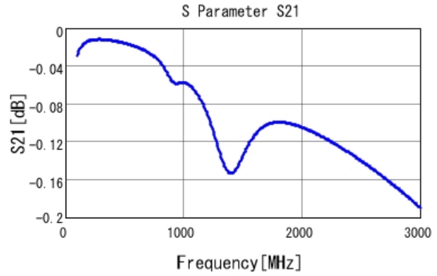
GRM21A7U2E221JW31 S21 DC0V, 25degC
