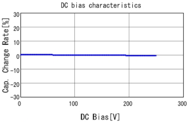
GRM21A7U2E221JW31 C-DC bias capchange, 25.0degC, A
