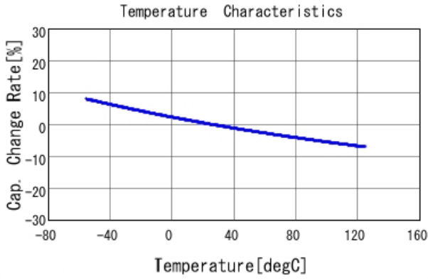
GRM21A7U2E221JW31 C-Temp. capchange, DC0V, AC1Vrms
