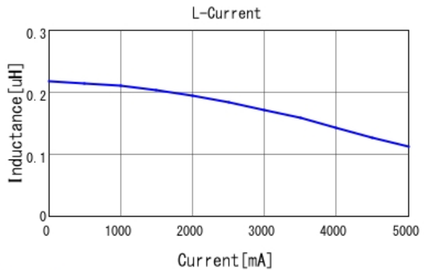
LQM2HPNR24MCH L-Current 20degC
