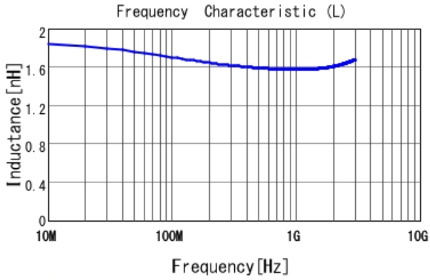
LQP03TG1N6C02 L
