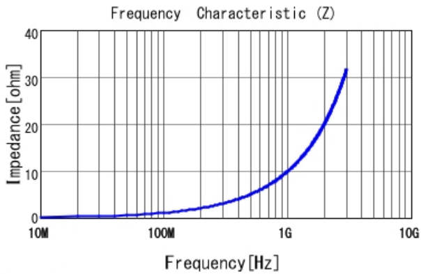
LQP03TG1N6C02 |Z|
