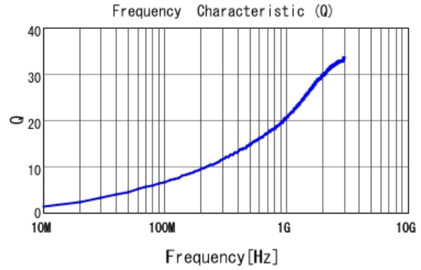
LQP03TG1N6C02 Q
