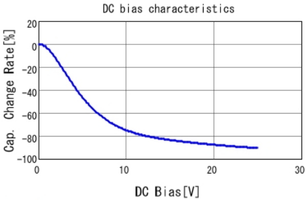
GRM033R61E104ME14 C-DC bias capchange, 25.0degC, A
