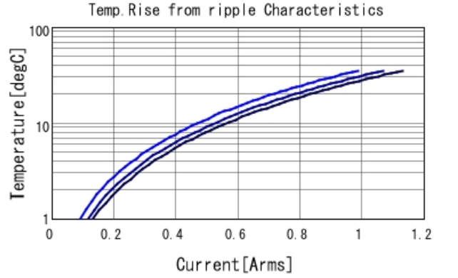
GRM033R61E104ME14 Temp. rise — 400kHz — 800I
