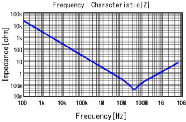
GRM033R61E104ME14 |Z| DCOV, 25degC
