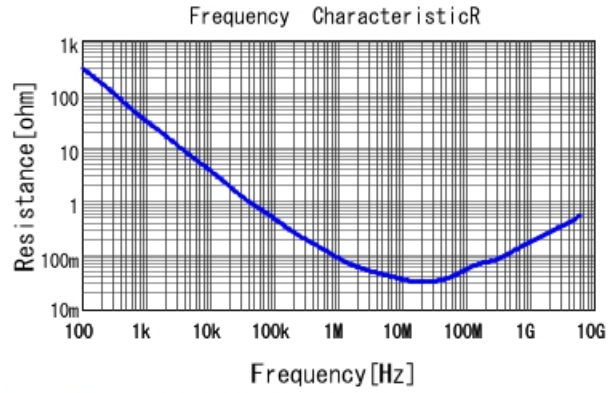
GRM033R61E104ME14 R DCOV, 25degC
