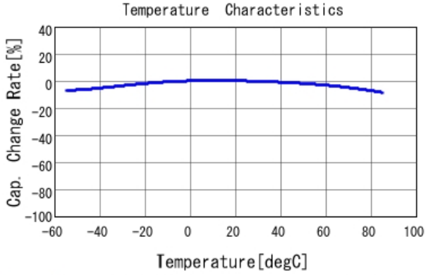
GRM033R61E104ME14 C-Temp. capchange, DC0.0V, AC0.5
