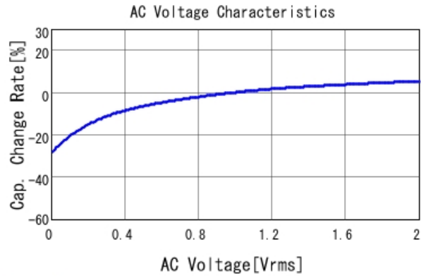
GRM033R61E104ME14 C-AC Voltage capchange, DCOV, 25
