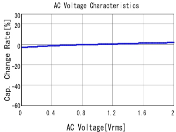
■ GRM188R72A103KA01 C-AC Voltage capchange, DCOV, 25.0d
