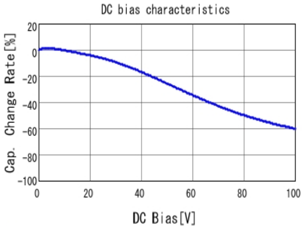
■ GRM188R72A103KA01 C-DC bias capchange, 25.0degC, AC1.
