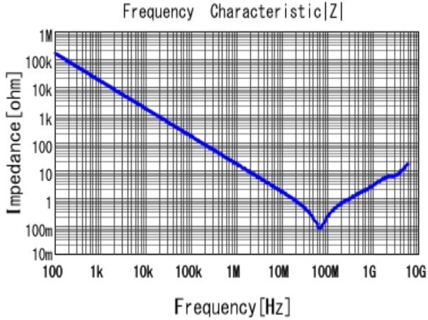
■ GRM188R72A103KA01 |Z| DCOV, 25degC
