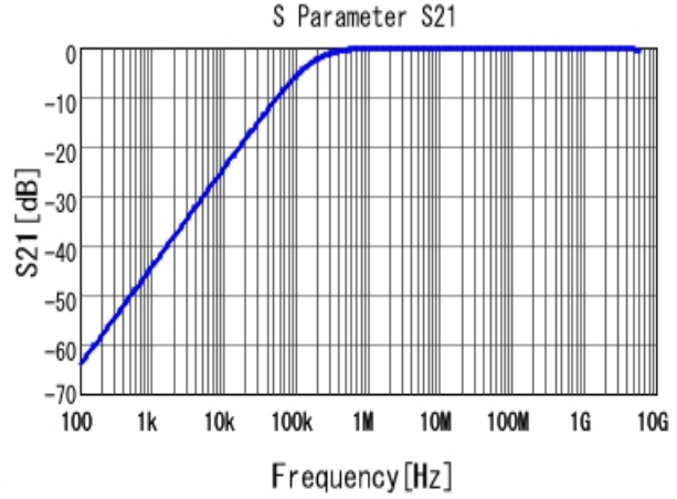
■ GRM188R72A103KA01 S21 DCOV, 25degC
