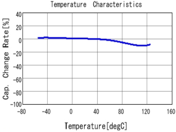
■ GRM188R72A103KA01 C-Temp. capchange, DCO. 0V, AC1.0Vrm
