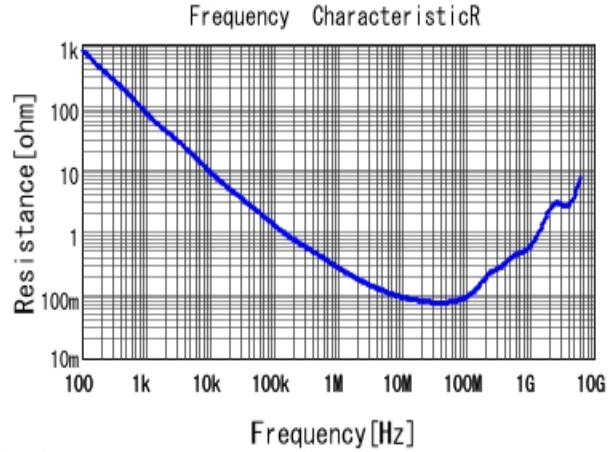
■ GRM188R72A103KA01 R DCOV, 25degC
