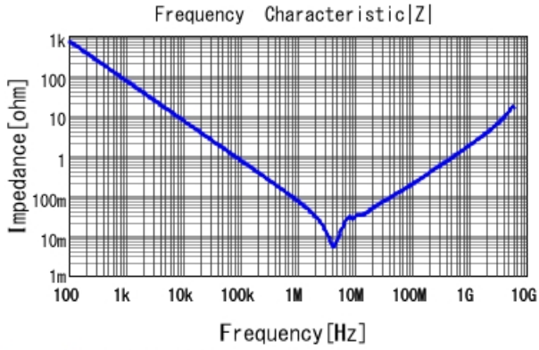
GRM21BR70J225KA01 |Z| DCOV, 25degC
