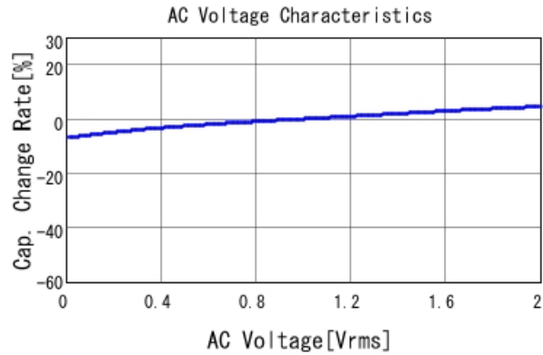
GRM21BR70J225KA01 C-AC Voltage capchange, DCOV, 25
