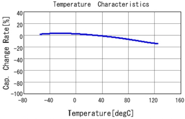
GRM21BR70J225KA01 C-Temp. capchange, DC0.0V, AC1.C
