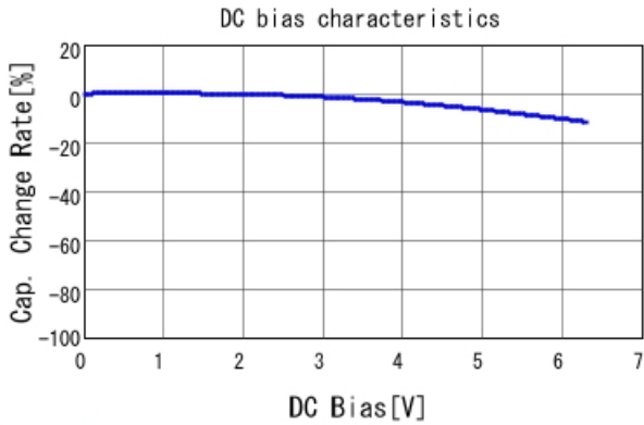
GRM21BR70J225KA01 C-DC bias capchange, 25.0degC, A
